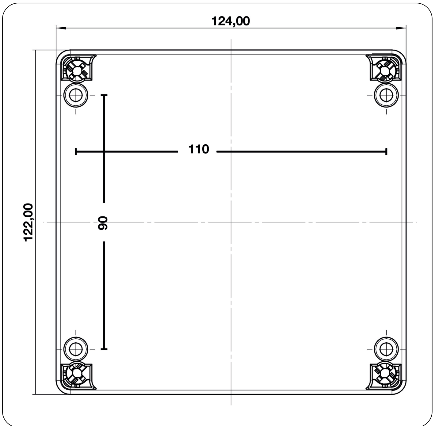
Fig.16 Mounting template
